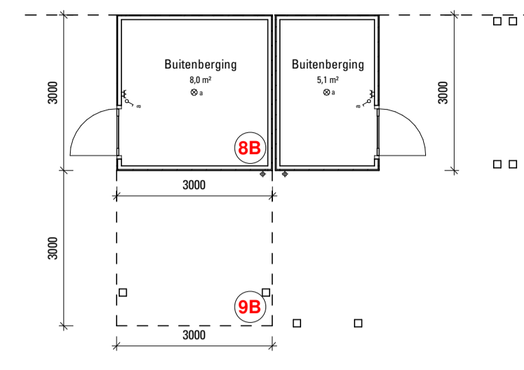
Begane grond 9B 1:100
